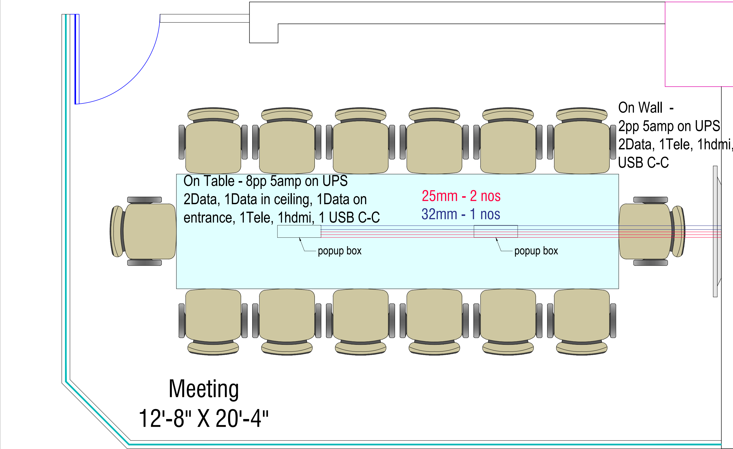
Typical detail-2 - Electrical and Data Point per Table
